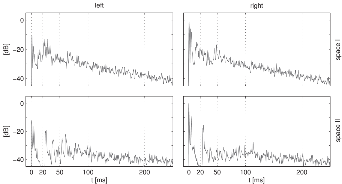
Figure 1: Energy envelopes of the binaural room impulse responses.
